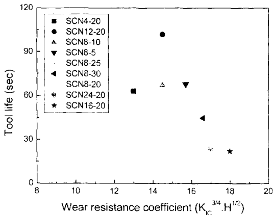
Fig. 10 Relation between wear resistance coefficient ( K_{IC}^{3/4}H^{1/2} , K_{IC} =fracture toughness, H =hardness) and tool life during machining gray cast iron at 330 m/min with a feed rate of 0.2 mm/rev and a depth of cut of 0.5 mm
