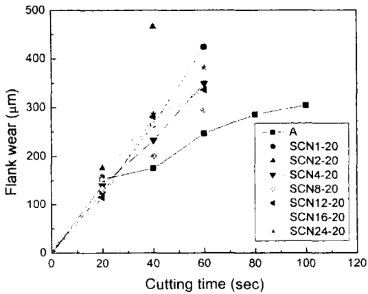
Fig. 3 Flank wear curves of SCN-series with different sintering time during machining heat-treated AISI4140 at 160 m/min with a feed rate of 0.2 mm/rev and a depth of cut of 0.25 mm
