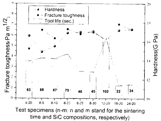
Fig. 8 Relation between mechanical properties (fracture toughness and hardness) and tool life during machining gray cast iron at 330 m/min with a feed rate of 0.2 mm/rev and a depth of cut of 0.5 mm
